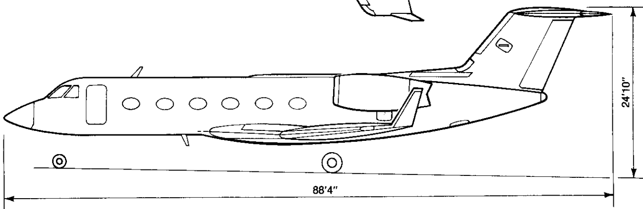
GULFSTREAM IV-SP
