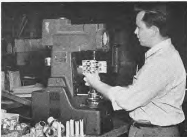
Heat-treated parts are carefully checked by Navy; Inspector Joseph Fry is taking a Rockwell hardness reading of a part before acceptance
