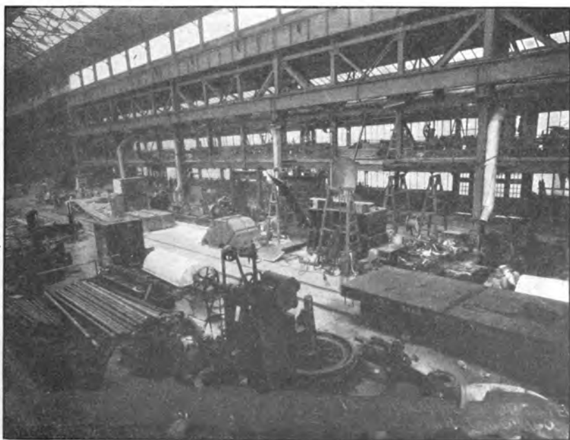
Interior of extension to heavy machine shop, Navy Yard, New York, N. Y.
