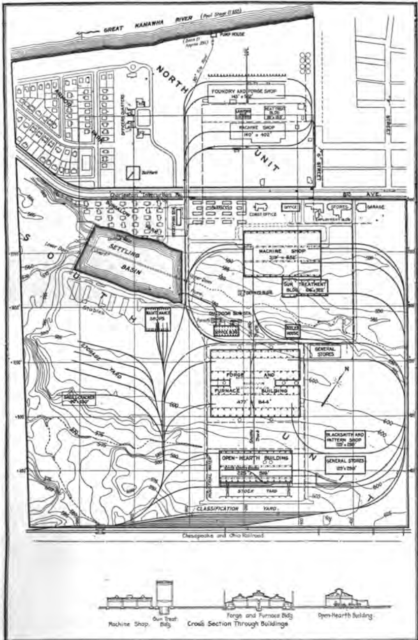
Plot plan of Naval Armor and Projectile Plants, Charleston, W. Va. [Reproduced by permission of American Society of Mechanical Engineers.]
