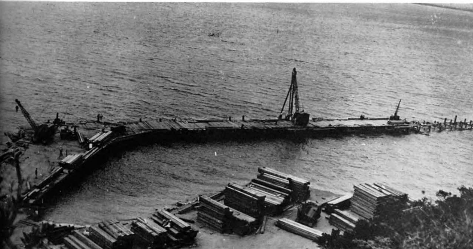
IMMEDIATELY PILE DRIVERS BEGIN OPERATIONS
