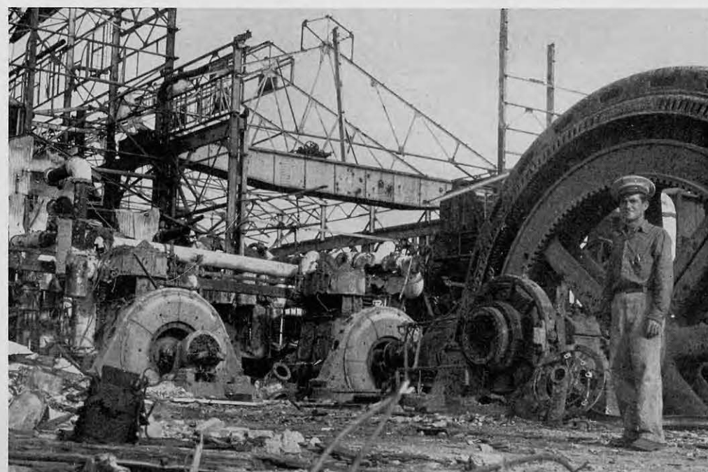
MODERN UNITS, MOSTLY FROM EUROPE, ONCE POWERED THIS GIANT MILL.
