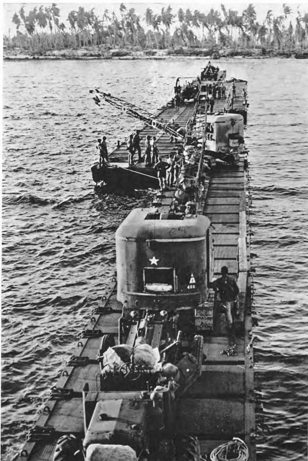
This LST-borne pontoon causeway went into use in the Marshall Islands invasion. The heavy gear brought in by the LSTs begins to move ashore. Note the side-rail fashion of joining the pontoon's sections together. When the equipment reaches the end of the last pontoon, "ducks" will drag it the rest of the way to shore.
