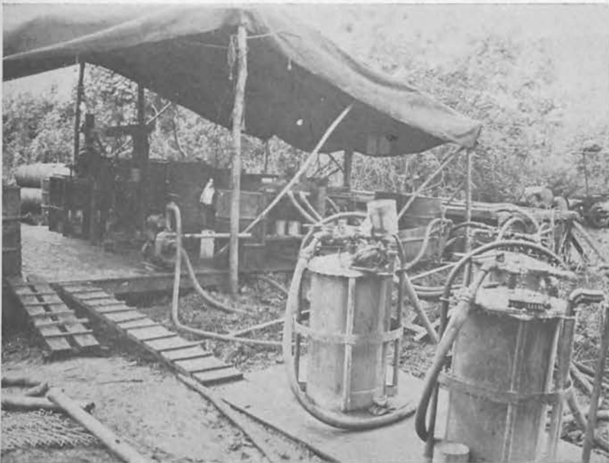
Water point to rear of camp. This is a stand by installation. Chlorinators are shown in the foreground with filters and sediment tank in the background.
