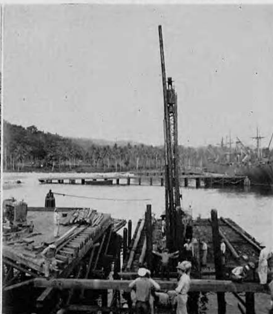
Here they are placing a 70-foot Spliced Piling in a Wharf
