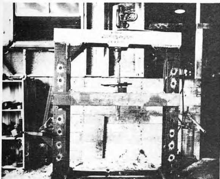
Transportation Department made a powerful hydraulic press from salvaged materials . . . .
